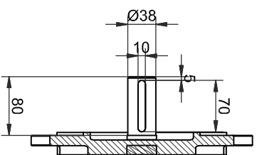
Shaft detail
